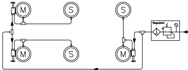
6 Isolator Piping Diagram
