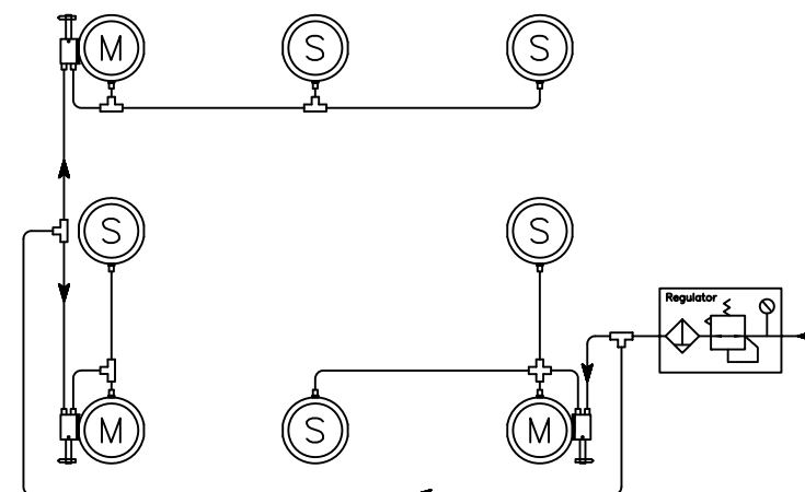
8 Isolator Piping Diagram
