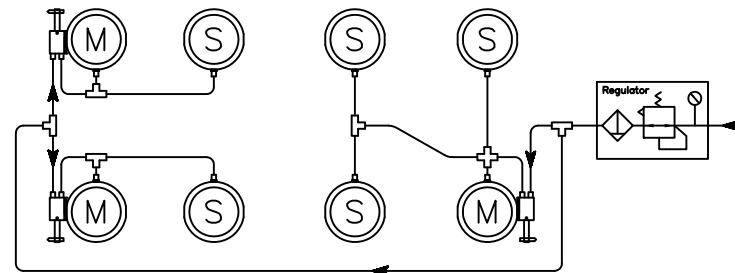
8 Isolator Piping Diagram
